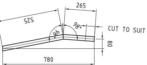
40x40x16 SHS MIRROR OF DETAIL: 2
